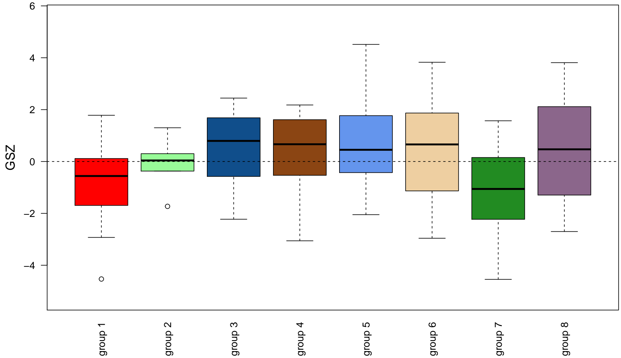
response to muscle stretch
